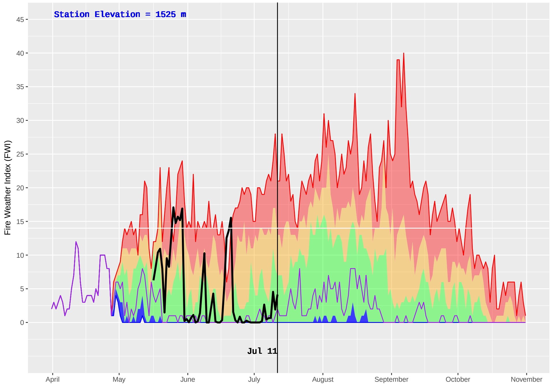
HARBOUR LAKE (250) : Historical (1989–2016) and Current (2018) Noon Fire Weather Index (FWI)
