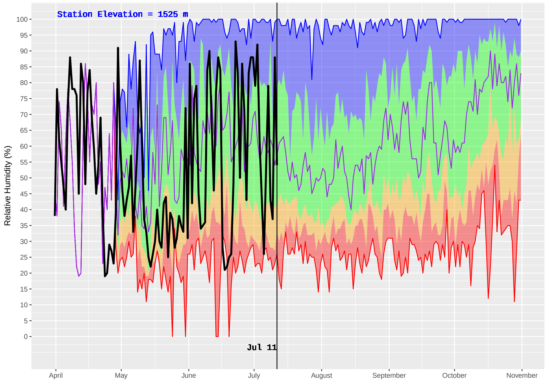
HARBOUR LAKE (250) : Historical (1989–2016) and Current (2018) Noon Relative Humidity
