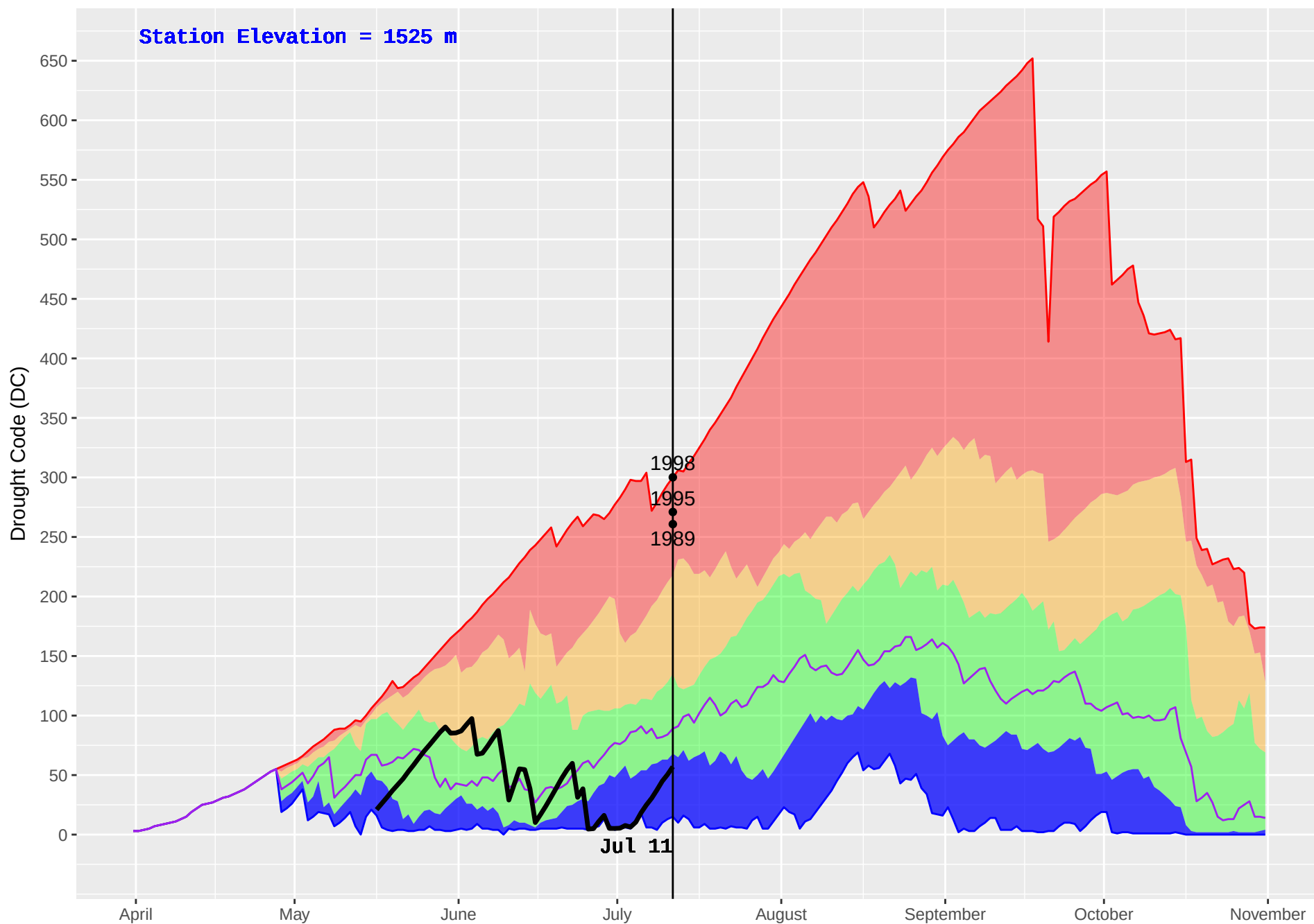
HARBOUR LAKE (250) : Historical (1989–2016) and Current (2018) Noon Drought Code (DC)
