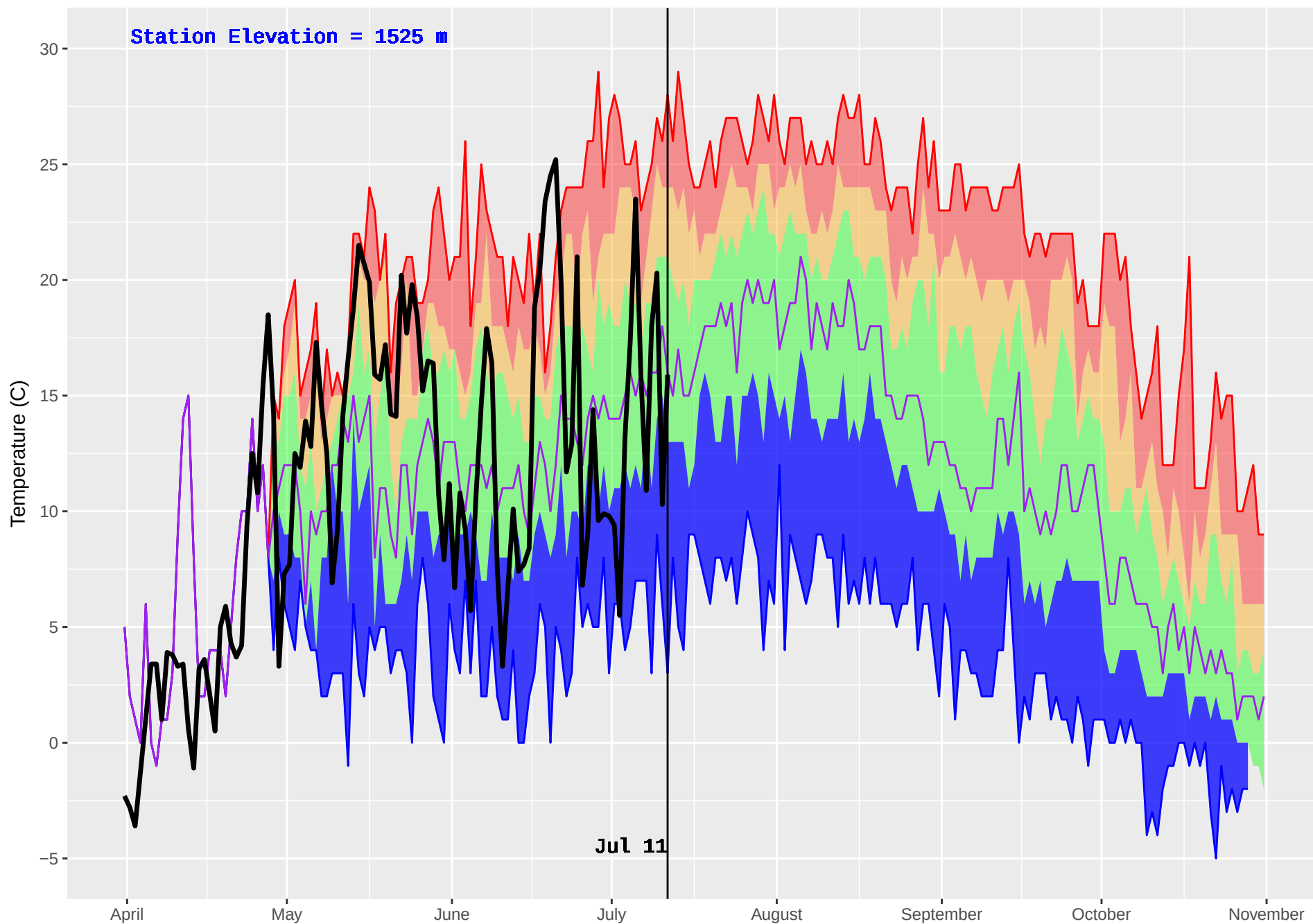
HARBOUR LAKE (250) : Historical (1989–2016) and Current (2018) Noon Temperature
