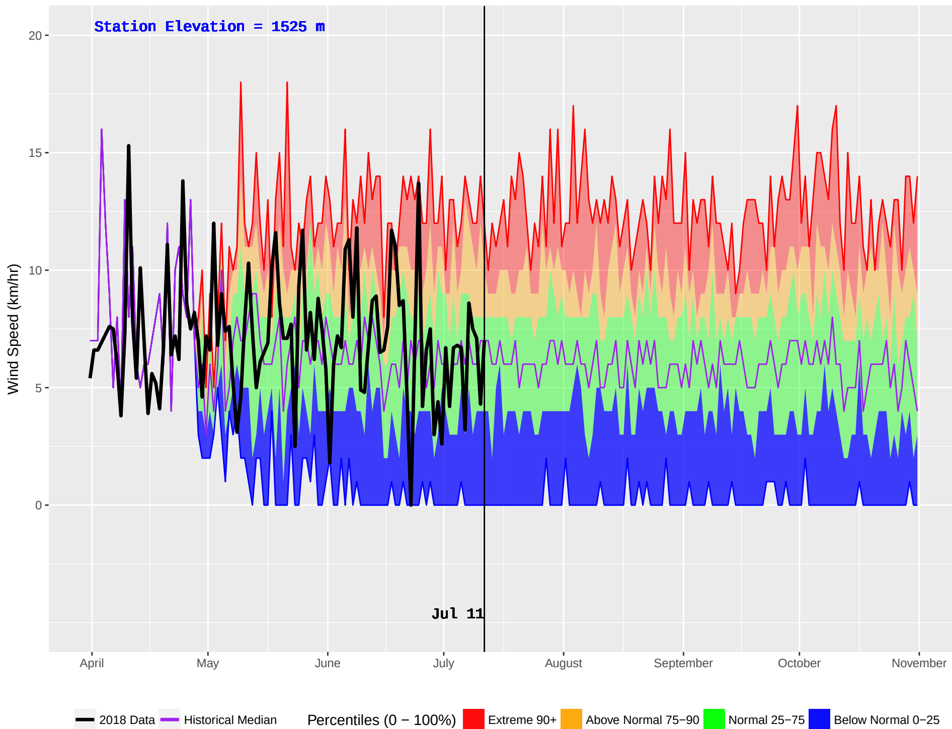
HARBOUR LAKE (250) : Historical (1989–2016) and Current (2018) Noon Wind Speed
