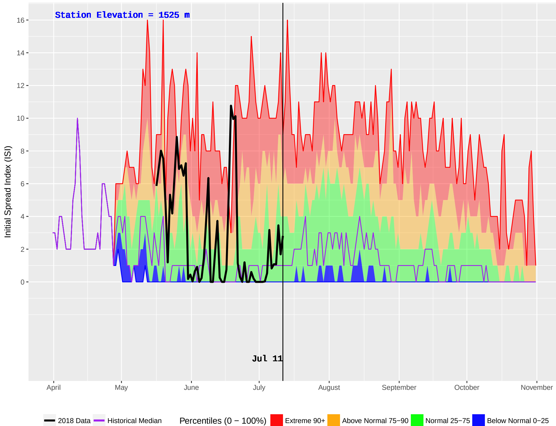
HARBOUR LAKE (250) : Historical (1989–2016) and Current (2018) Noon Initial Spread Index (ISI)
